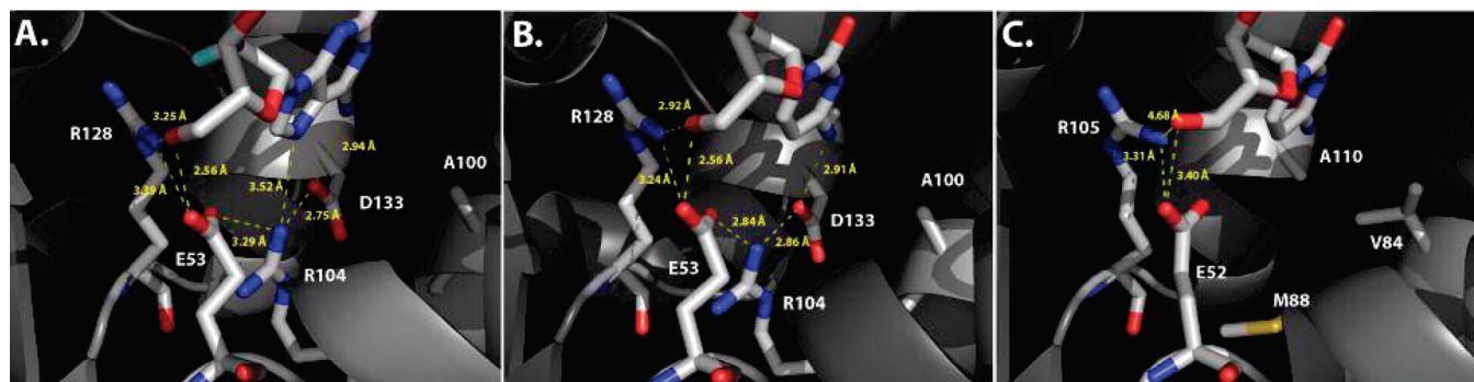
FIGURE 1: Active site comparison of human dCK and DmdNK with pyrimidine and purine nucleoside substrates. Detailed view of the active sites of dCK in the presence of the 2'-deoxyadenosine analogue clofarabine (A; PDB code: 2A7Q (13) and dC (B; PDB code: 1P6O (11)), as well as DmdNK with dC (C; PDB code: 1J90 (9)). In all three enzymes, the nucleoside is bound in the phosphoryl-acceptor site. Hydrogen-bonding interactions between the substrate's 5'-hydroxyl group, Arg128 (Arg105 in DmdNK ) and Glu53 (Glu52) are highly conserved. The latter functions as a general base in the phosphoryl transfer reaction. In dCK, both purine and pyrimidine nucleosides form an elaborate network of hydrogen bonds between Glu53 and the exocyclic amino group on the substrate nucleobase, involving Arg104 and Asp133. The same residues in DmdNK , Met88 and Ala110, create a significantly larger binding pocket with no specific contacts, presumably allowing for the broader substrate specificity in the fruitfly enzyme. Position Ala100 (Val84 in DmdNK ) flanks Asp133.
